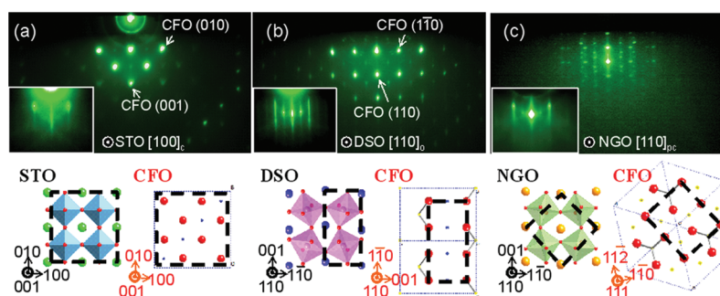
Figure 2. RHEED patterns and schematics of \text{CoFe}_2\text{O}_4 - \text{BiFeO}_3 films grown on (a) \text{SrTiO}_3 , (b) \text{DyScO}_3 , and (c) \text{NdGaO}_3 (001) _c -oriented substrates. The insets show the pattern of the corresponding substrate before film growth.
