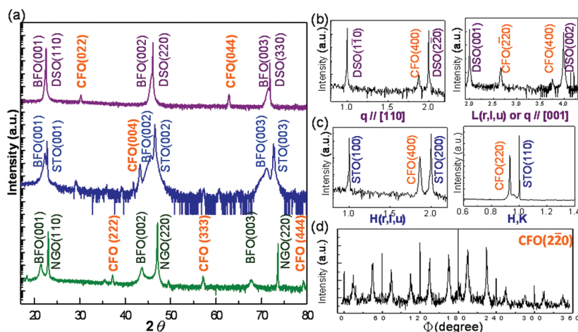
Figure 3. (a) Out-of-plane X-ray diffraction of \text{CoFe}_2\text{O}_4 - \text{BiFeO}_3 on different substrates. (b, c) In-plane XRD of films grown on the DSO and STO substrates. (d) Phi scan of CFO on NGO substrates.
